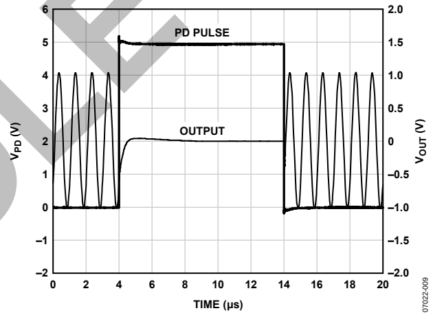
Figure 9. Power-Down/Power-Up Transition
