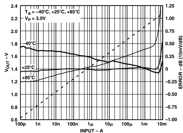
TPC 6. Logarithmic Conformance (Linearity) for a 3 V Single Supply (See Figure 6)
