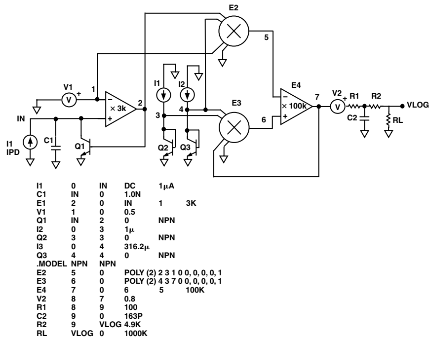
Figure 12. Basic Macromodel
