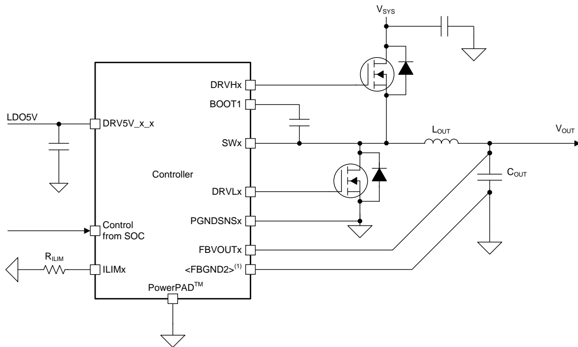
Figure 7-2. Controller Diagram
