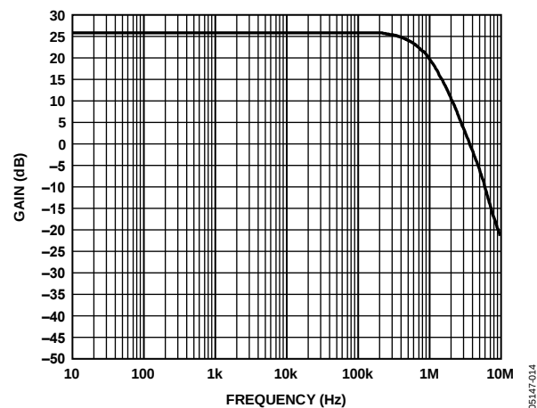
Figure 7. Typical Small Signal Bandwidth (Output Voltage ( V_{out} ) = 200 mV p-p)
