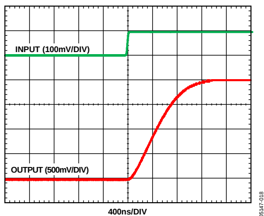
Figure 9. Rise Time
