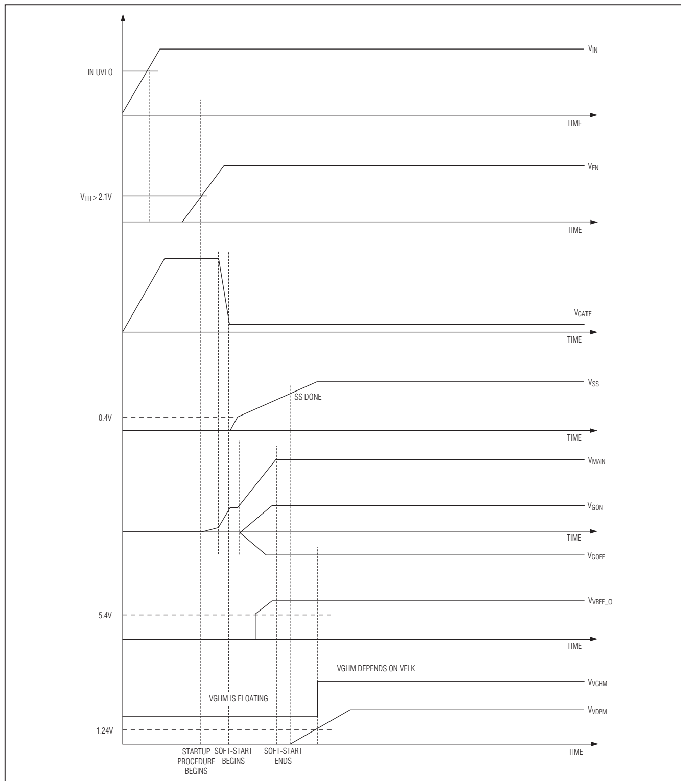
Figure 4. Power-Up Sequence
