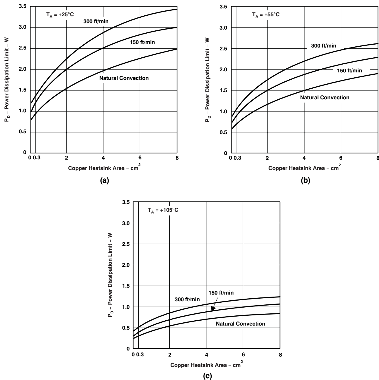
Figure 28. Power Ratings of the PWP Package at Ambient Temperatures of +25^\circ\text{C} , +55^\circ\text{C} , and +105^\circ\text{C}
