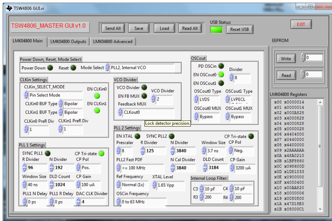
Figure 5. PLL2 Settings
