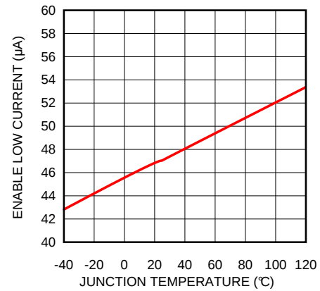
Figure 8. Enable Low Current vs Temperature
