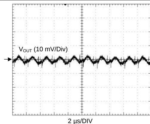
Figure 35. Output Voltage Ripple ( I_{\text{OUT}} = 15 \text{ A} )
