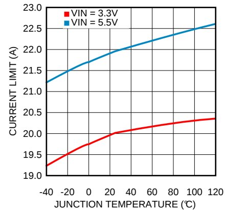
Figure 14. Peak Current Limit ( I_{CLR} ) vs Temperature
