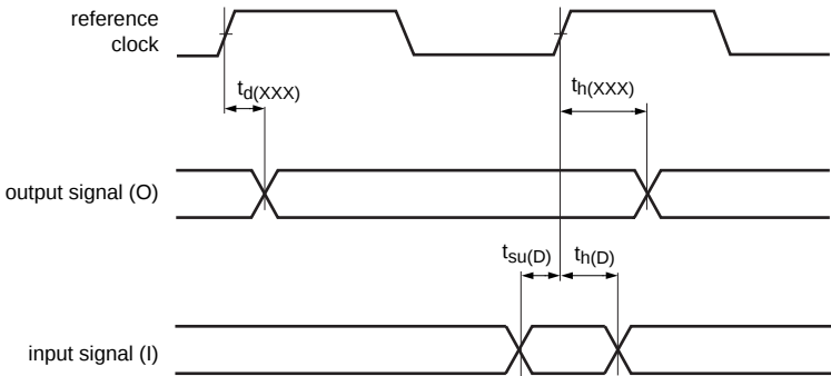
Fig 17. Signal timing
