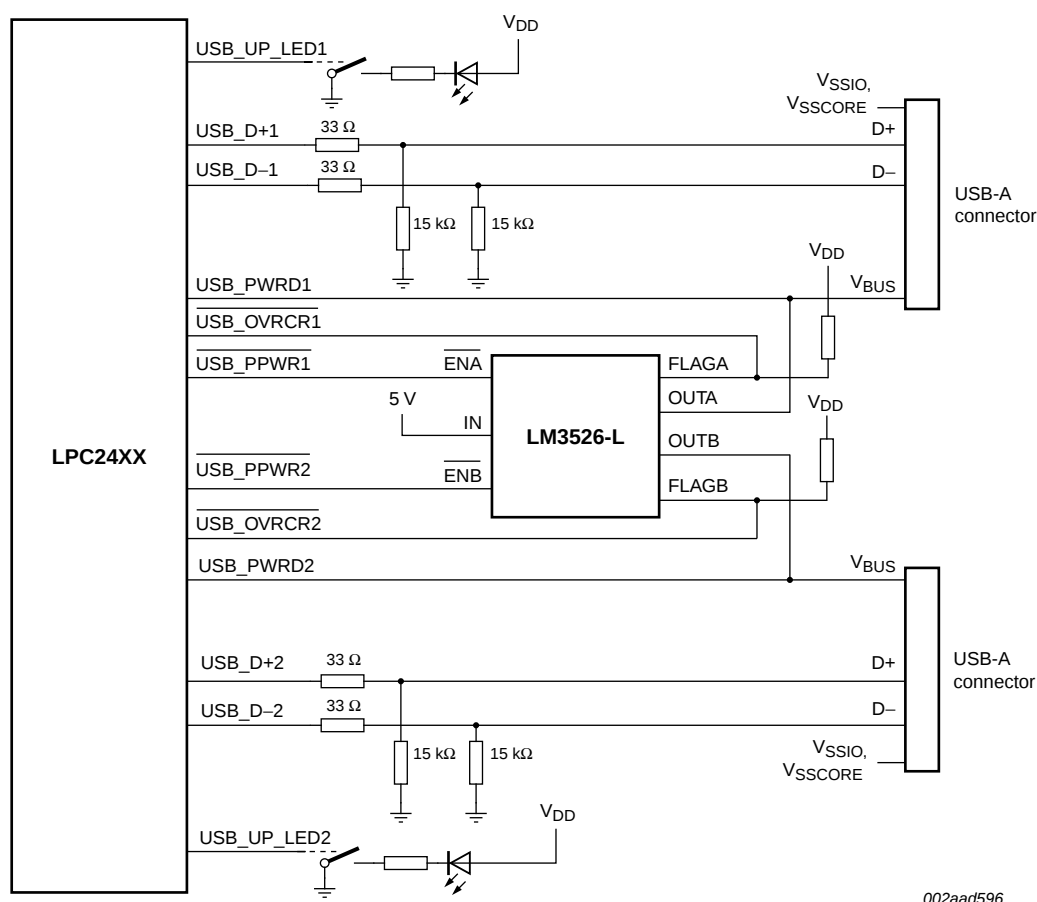
Fig 25. LPC2458 USB OTG port configuration: USB port 1 host, USB port 2 host
