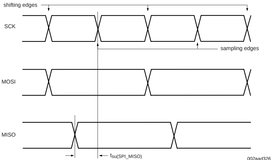
Fig 16. MISO line set-up time in SSP Master mode
