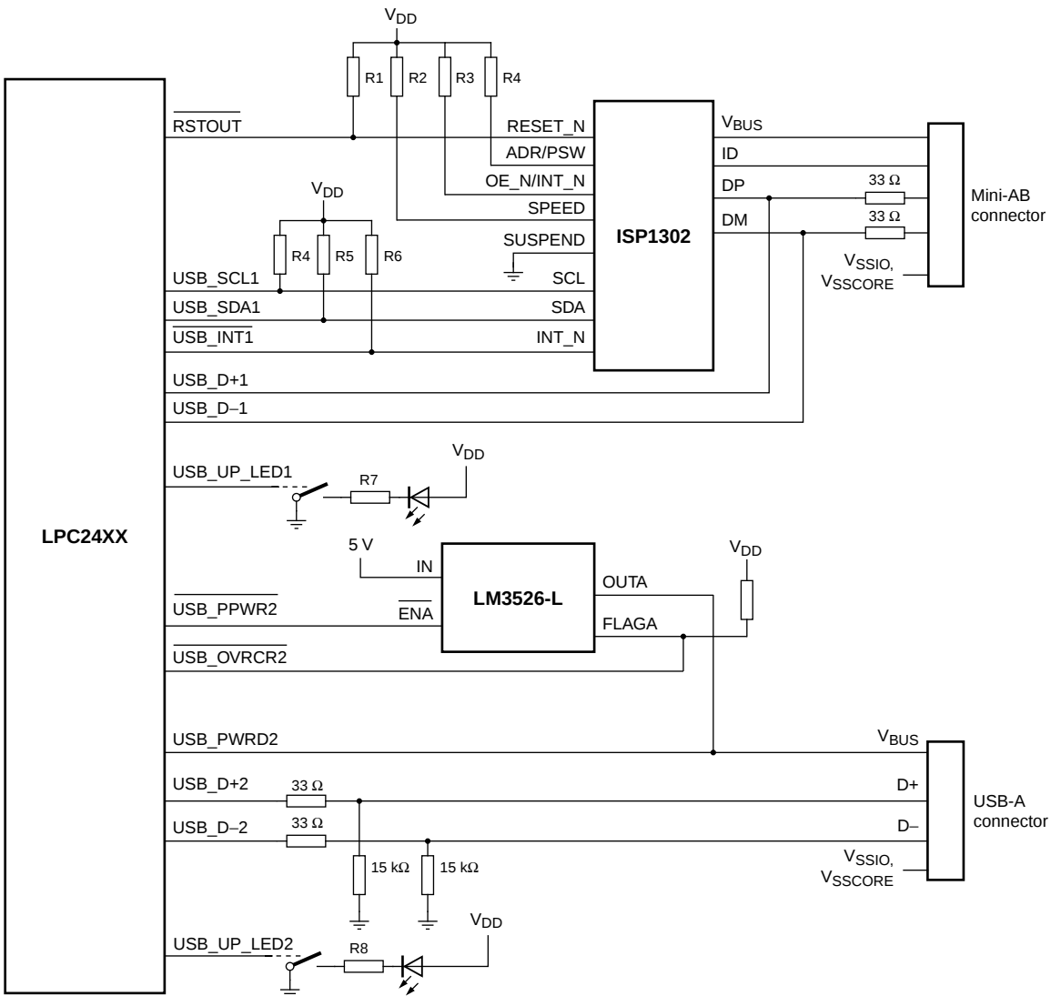
Fig 22. LPC2458 USB OTG port configuration: USB port 1 OTG dual-role device, USB port 2 host
