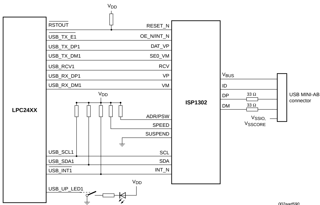
Fig 23. LPC2458 USB OTG port configuration: VP_VM mode
