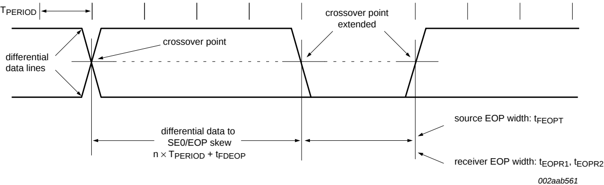
Fig 15. Differential data-to-EOP transition skew and EOP width
