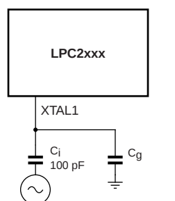
Fig 26. Slave mode operation of the on-chip oscillator
