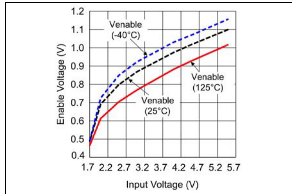
FIGURE 2-4: MIC94080/1 Enable Threshold vs. Input Voltage.
