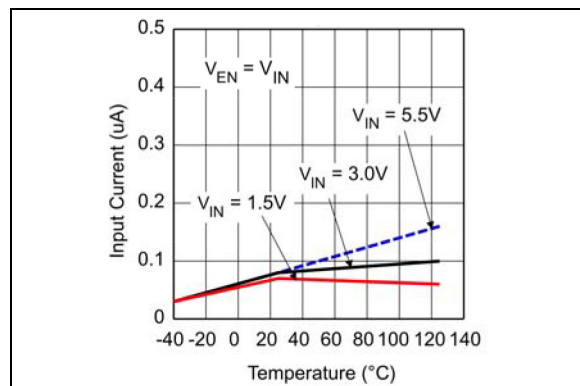
FIGURE 2-6: MIC94080/1 Input Current vs. Temperature.
