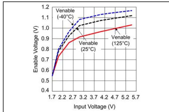
FIGURE 2-5: MIC94082/3/4/5 Enable Threshold vs. Input Voltage.
