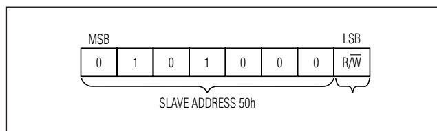
Figure 1. DS3503 Slave Address Byte
