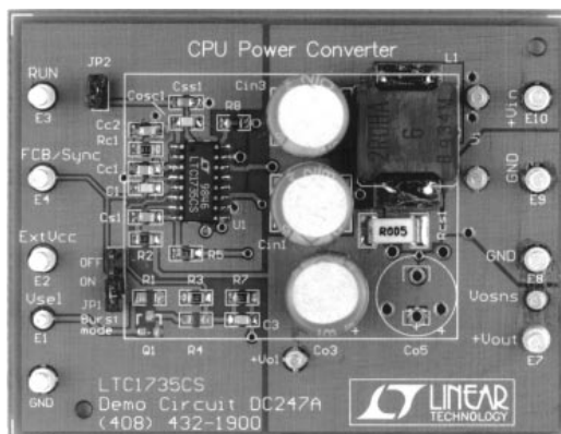
Demo Circuit 247A
