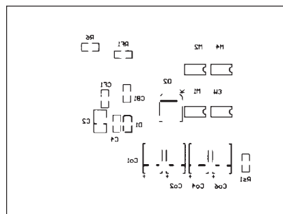
Bottom Side Silkscreen
