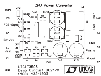
Top Side Silkscreen
