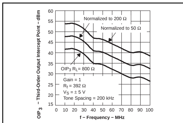
Figure 111. Equivalent 3rd-Order Intercept Point for the THS4500
