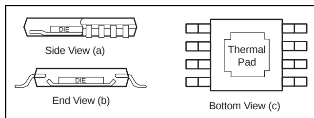
Figure 113. Views of PowerPAD, Thermally-Enhanced Package
