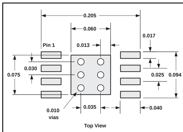
Figure 114. PowerPAD PCB Etch and Via Pattern
