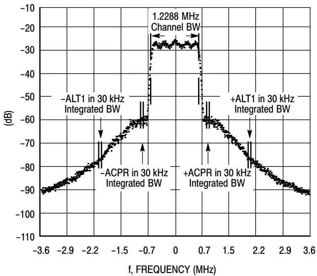
Figure 11. Single-Carrier N-CDMA Spectrum
