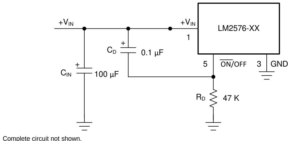
Figure 22. Delayed Start-Up
