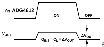
Figure 27. Charge Injection
