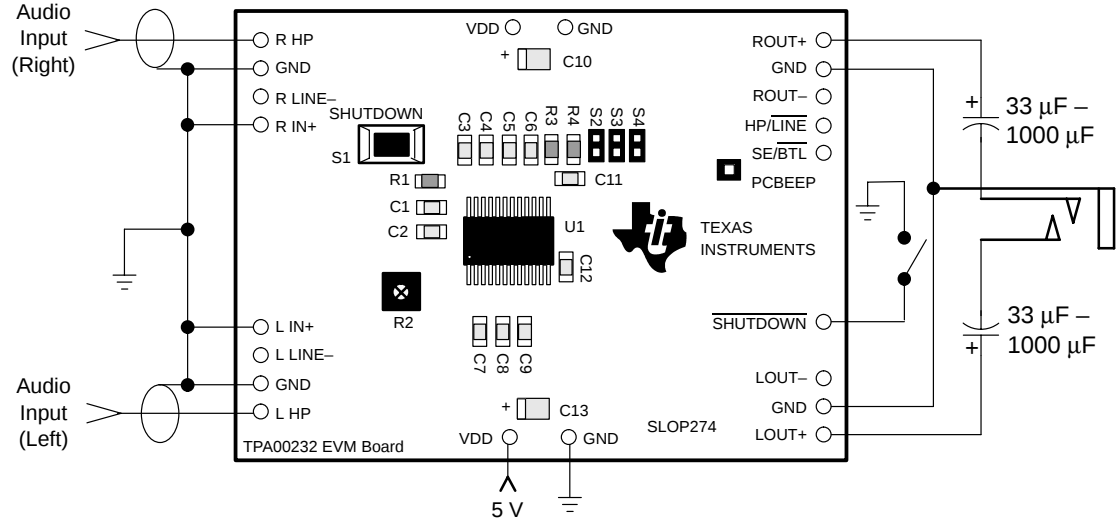
Figure 3–10. TPA0232 EVM Connected for Stereo Single-Ended Output
