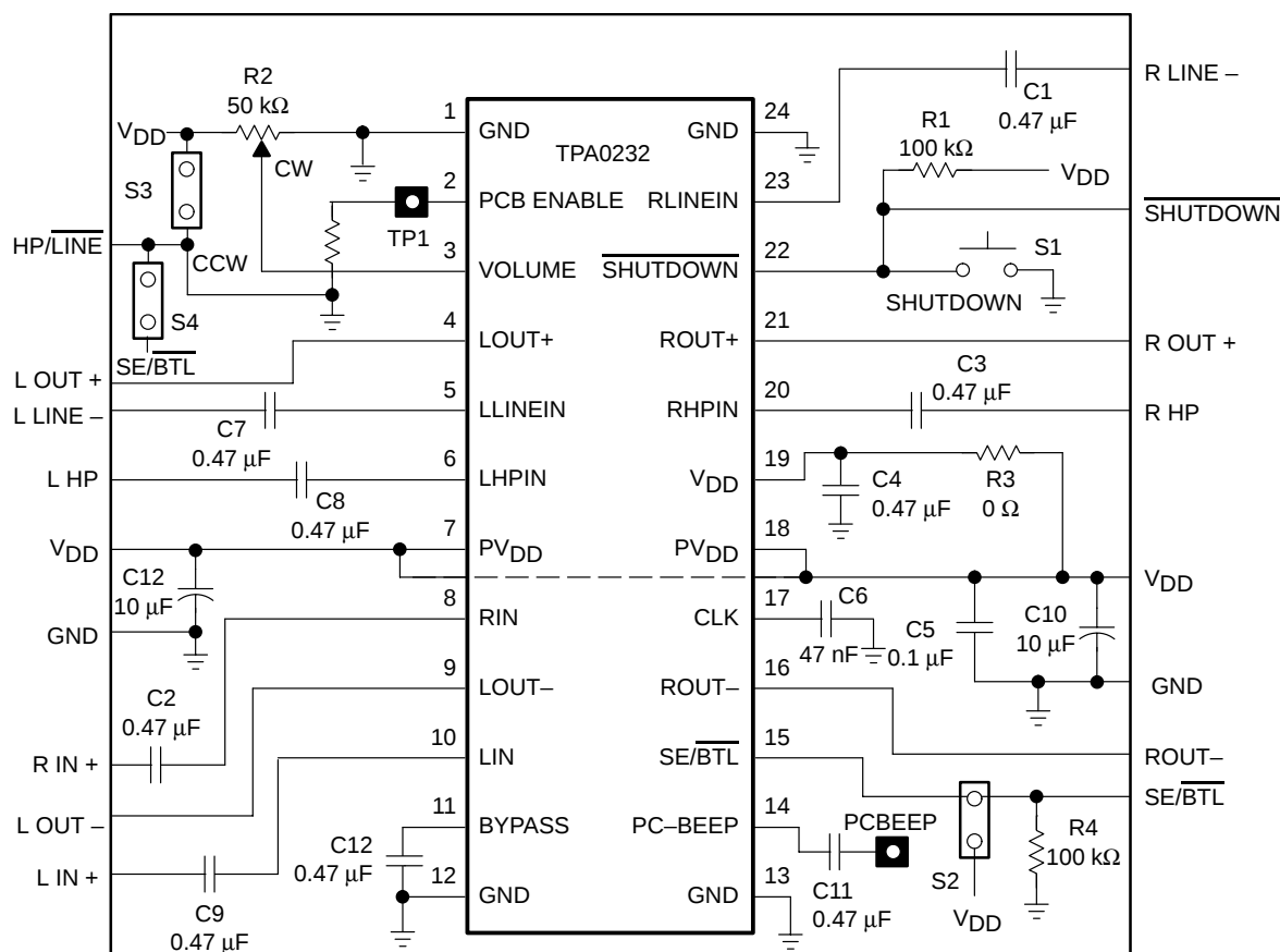
Figure 3–3. TPA0232 EVM Schematic Diagram
