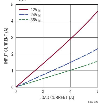
LTM8053 Input vs Load Current V_{OUT} = 8\text{V} , BIAS = 5V
