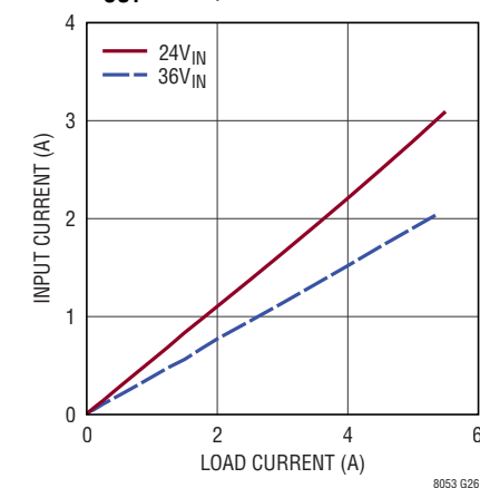
LTM8053 Input vs Load Current V_{OUT} = 12\text{V} , BIAS = 5V
