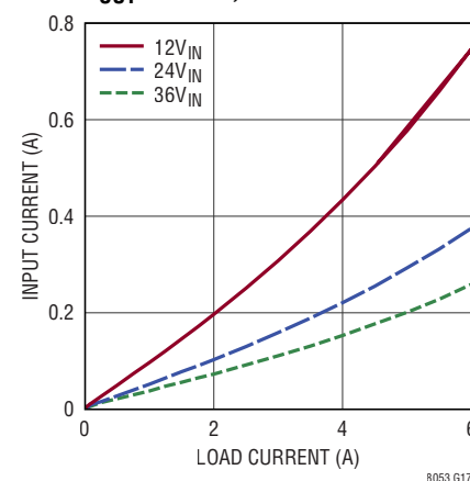
LTM8053 Input vs Load Current V_{OUT} = 0.97\text{V} , BIAS = 5V
