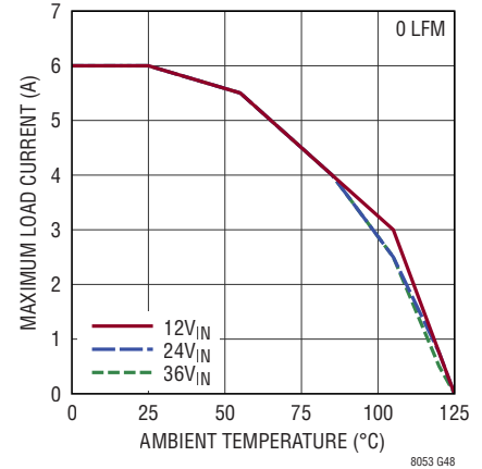
LTM8053 Derating, V_{OUT} = 0.97\text{V} , BIAS = 5V, DC1934A Demo Board
