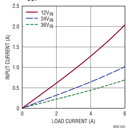
LTM8053 Input vs Load Current V_{OUT} = 3.3\text{V} , BIAS = 5V
