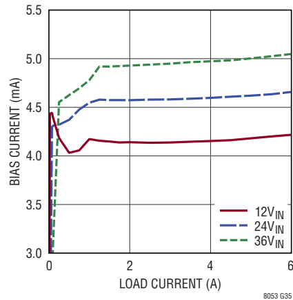
LTM8053 BIAS Current vs Load Current V_{OUT} = 1.5\text{V} , BIAS = 5V
