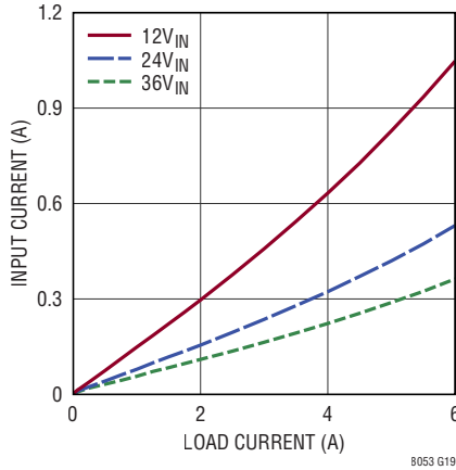
LTM8053 Input vs Load Current V_{OUT} = 1.5\text{V} , BIAS = 5V
