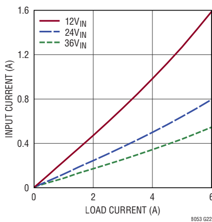
LTM8053 Input vs Load Current V_{OUT} = 2.5\text{V} , BIAS = 5V
