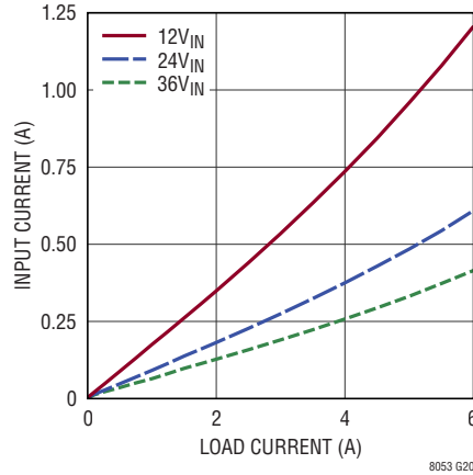
LTM8053 Input vs Load Current V_{OUT} = 1.8\text{V} , BIAS = 5V
