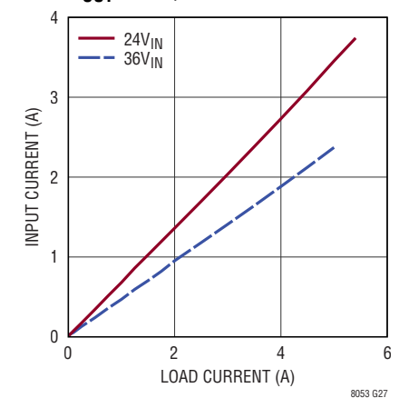
LTM8053 Input vs Load Current V_{OUT} = 15\text{V} , BIAS = 5V
