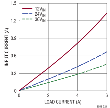
LTM8053 Input vs Load Current V_{OUT} = 2\text{V} , BIAS = 5V
