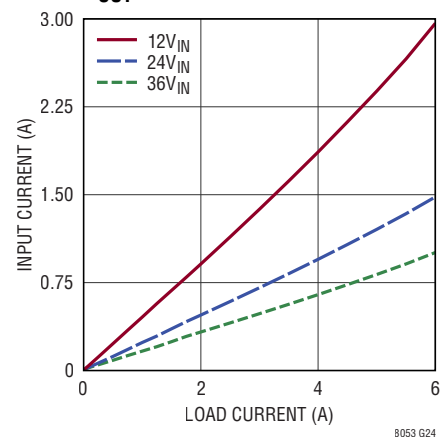
LTM8053 Input vs Load Current V_{OUT} = 5\text{V} , BIAS = 5V
