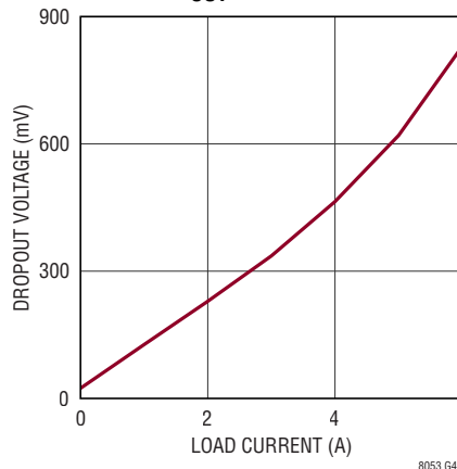
LTM8053 Dropout Voltage vs Load Current, V_{OUT} = 5\text{V} , BIAS = 5V
