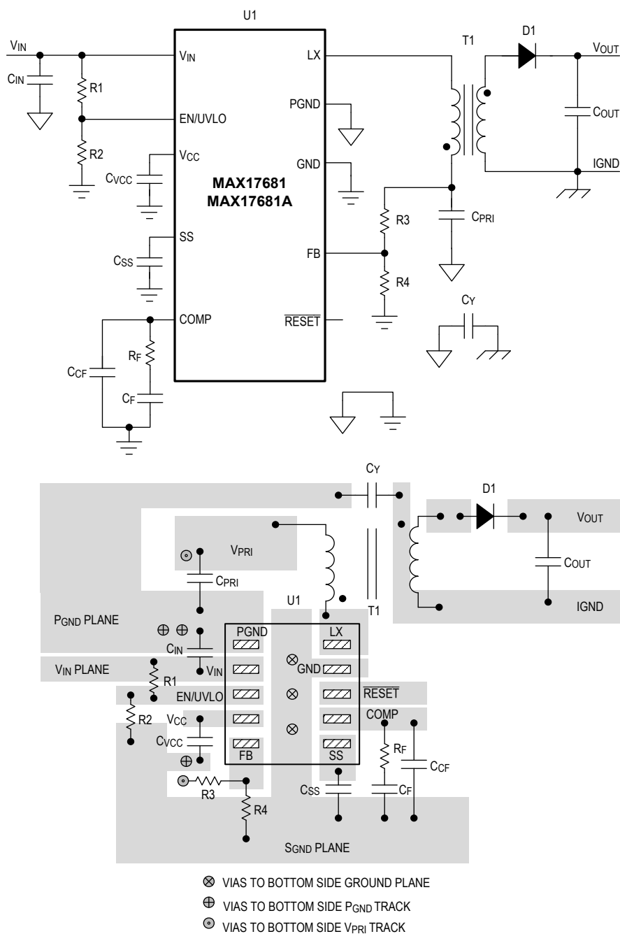
Figure 8. Recommended Component Placement
