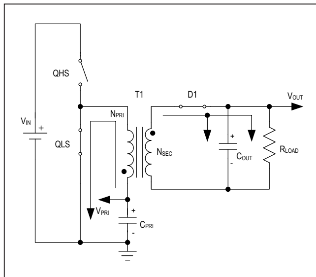
Figure 3. Off-Period Equivalent Circuit
