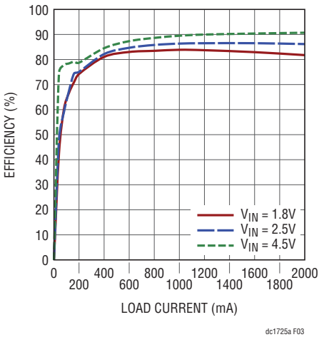
Figure 3. Efficiency with Different Input Voltages
