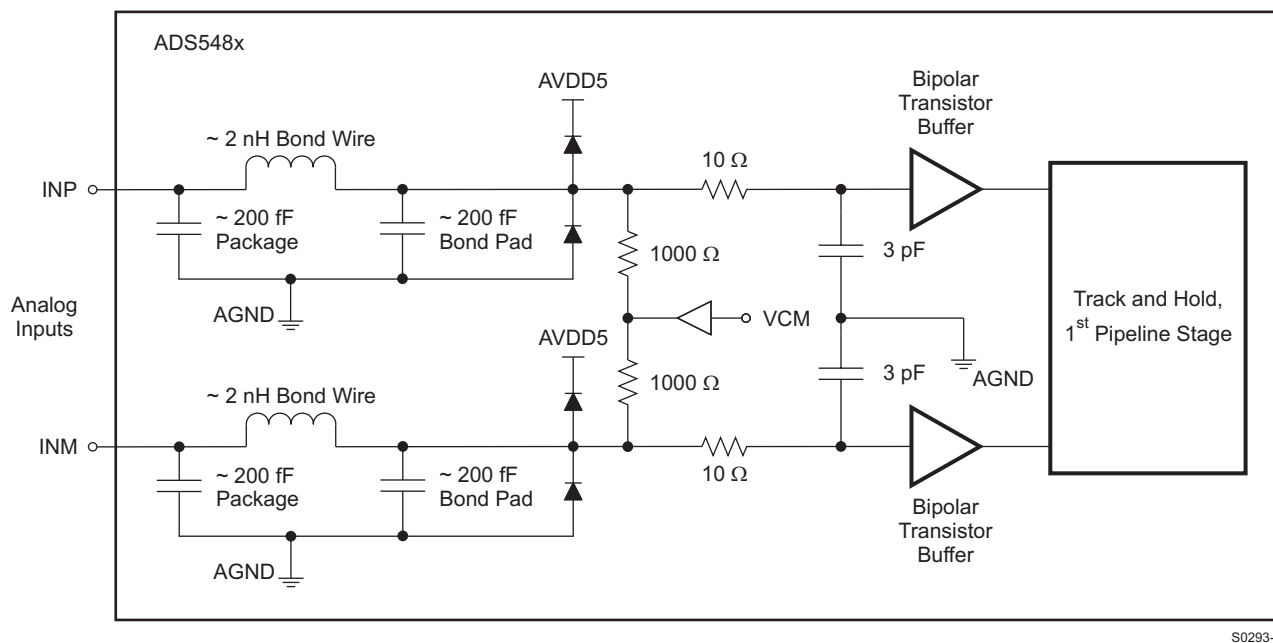
Figure 60. Analog Input Circuit
