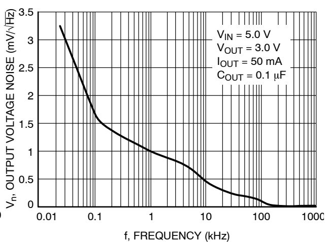
Figure 12. Output Voltage Noise
