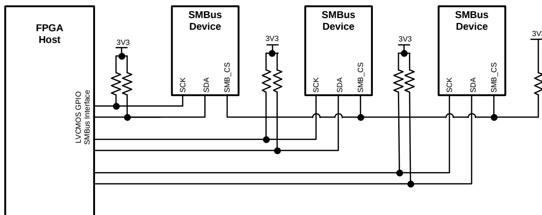
Figure 11. SMBus Configuration 3 — Host to multiple devices with multiple SMBus Interfaces
