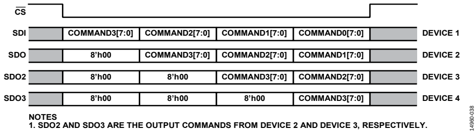
Figure 44. Example of an SPI Frame Where Four ADGS1412 Devices Connect in Daisy-Chain Mode
