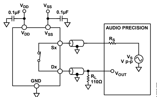
Figure 33. THD + Noise
