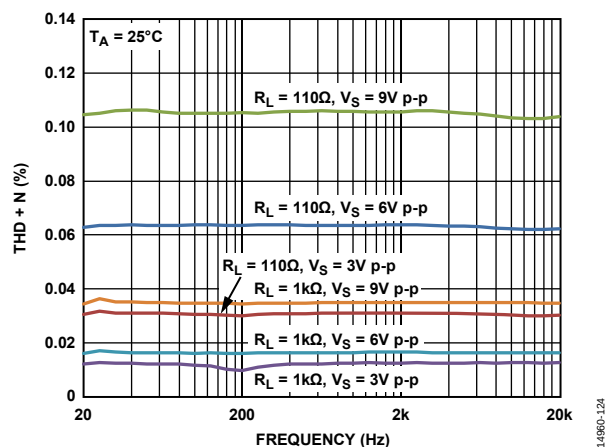
Figure 24. THD + N vs. Frequency, 12 V Single Supply
