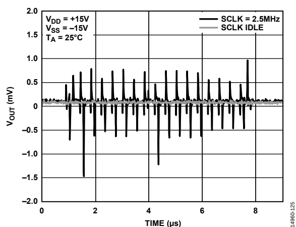
Figure 25. Digital Feedthrough
