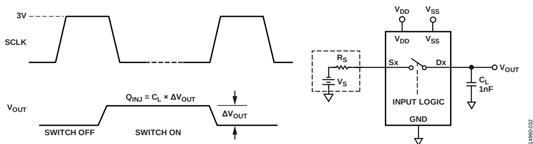
Figure 38. Charge Injection, Q_{INJ}
