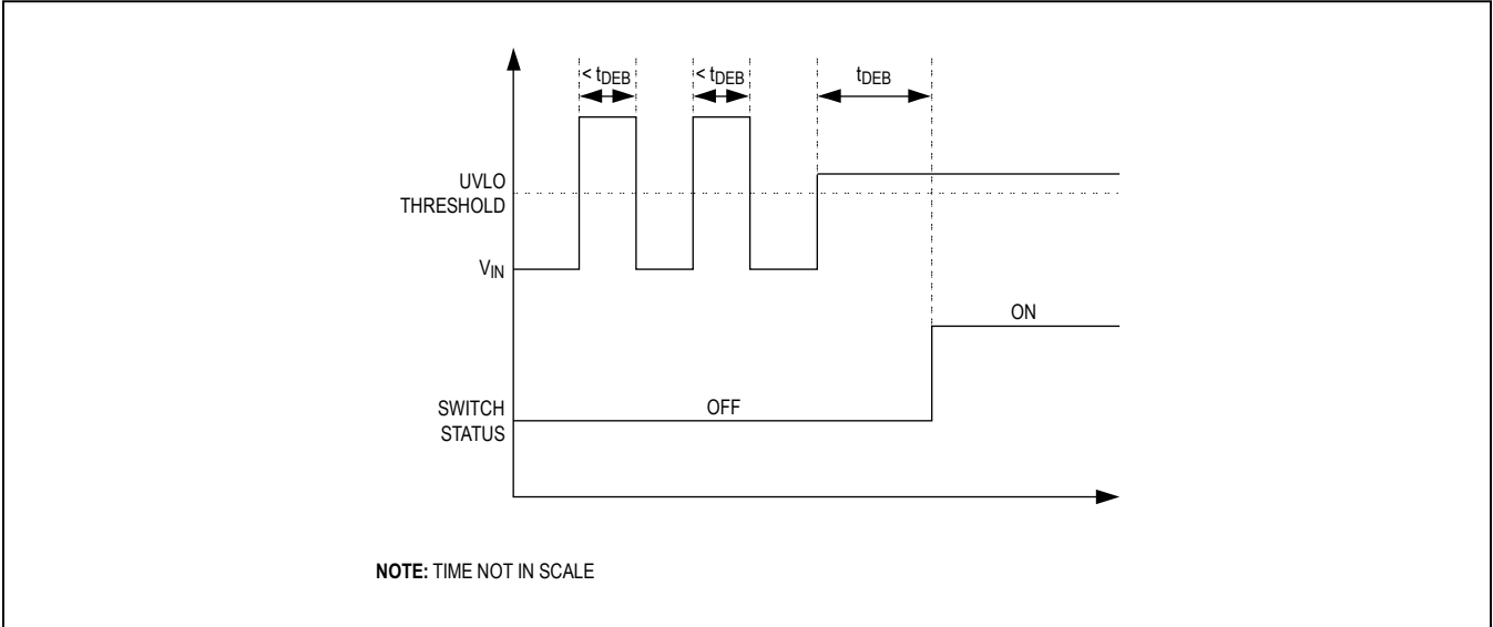
Figure 4. Debounce Timing
