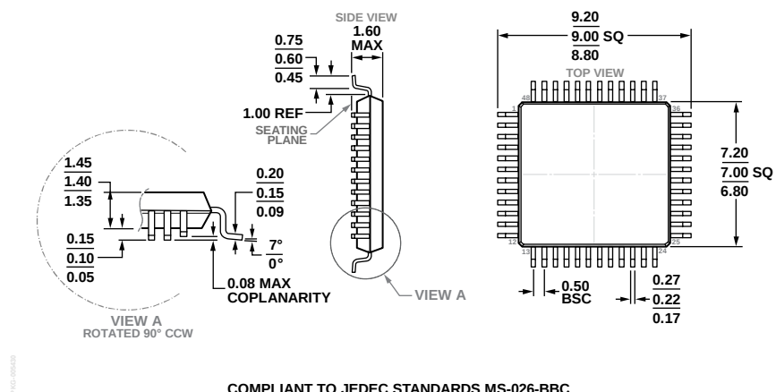
Figure 9. 48-Lead Low Profile Quad Flat Package [LQFP] (ST-48)
