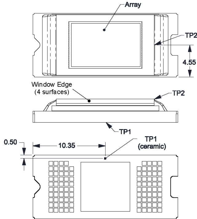
Figure 8. Thermal Test Point Location - FQD Package
