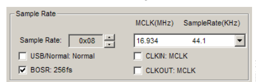
Figure 20. Sample Rate Control Section
