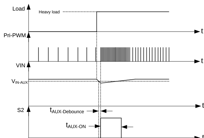
Figure 15 VIN-UVP Protection
