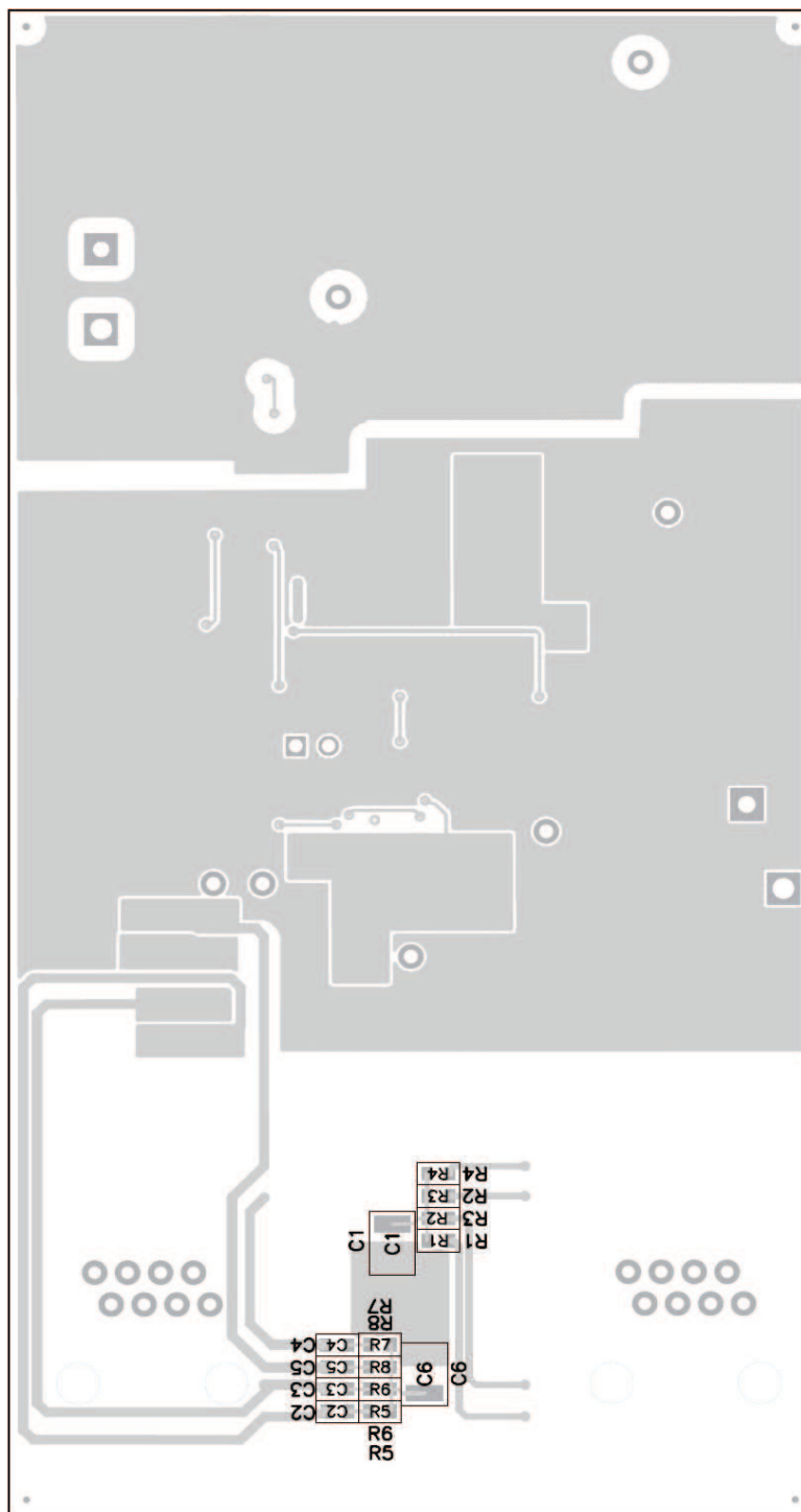
Figure 7. Bottom-Side Layout
