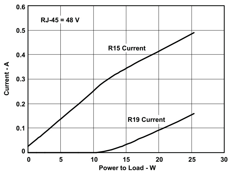
Figure 4. Booster Circuit Current Distribution
