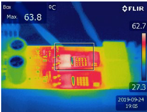
Figure 3. Thermal Image of Power Transistors (Both Channels Active, 16 LEDs in the String – Power 55 W)
