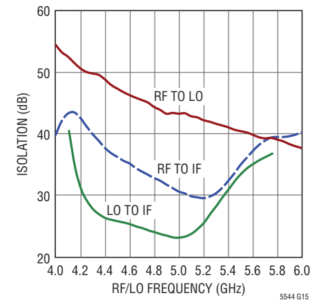
RF/LO Isolation
