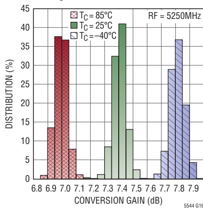
5250MHz Conversion Gain Histogram
