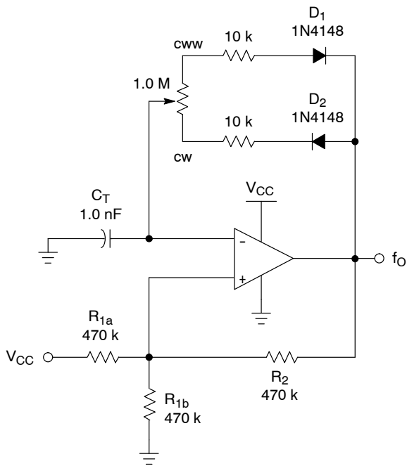
Figure 35. Variable Duty Cycle Pulse Generator
