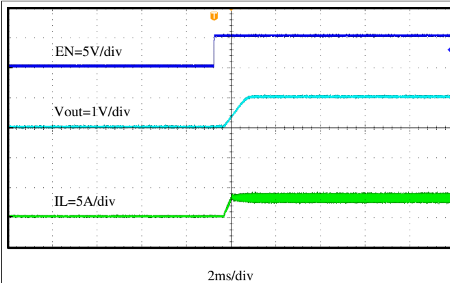
Figure 26. Start-Up Through EN, I_{OUT} = 3\text{ A}
