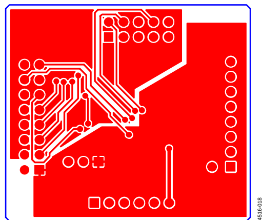
Figure 18. EVAL-AD5340DBZ Daughter Board Bottom Side Routing
