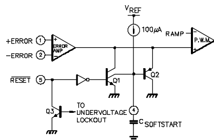
FIGURE 22. SOFT-START CIRCUIT SCHEMATIC
