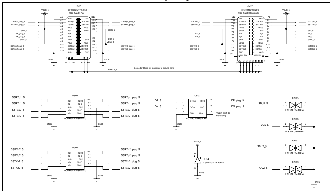
Figure 4: STEVAL-OET004V1D circuit schematic: protection and filtering solution with 500 \mu\text{m} and 0201 packages
