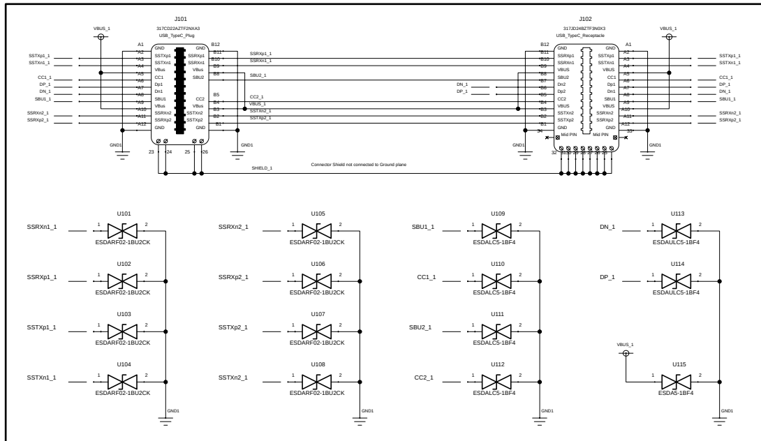
Figure 2: STEVAL-OET004V1B circuit schematic: protection solution with 400 \mu m packages
