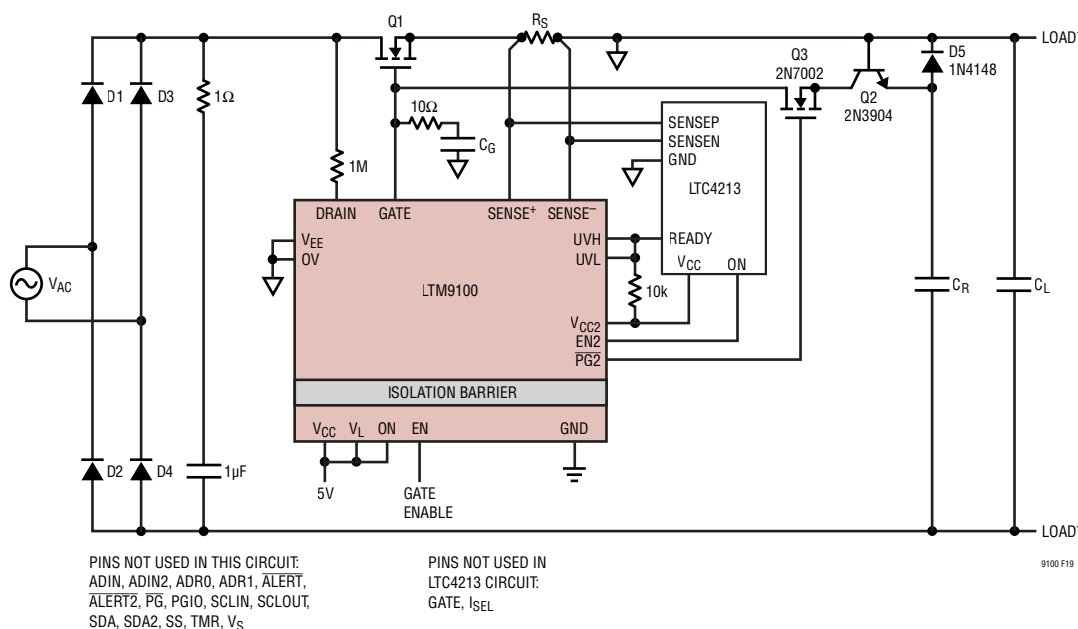
Figure 19. Rectified AC High Side Charging Circuit
