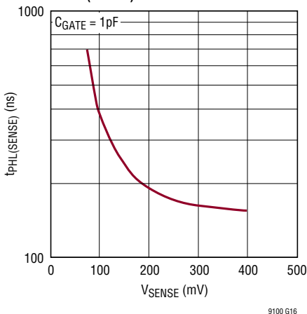
Current Limit Propagation Delay ( t_{\text{PHL(SENSE)}} ) vs V_{\text{SENSE}}
