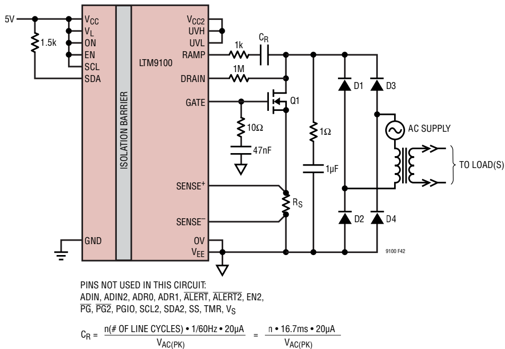
Figure 42. Transformer Inrush Current Limiter, n Line Cycle Ramp
