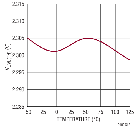
UVL Threshold vs Temperature
