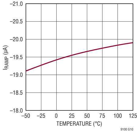
Ramp Pin Current vs Temperature
