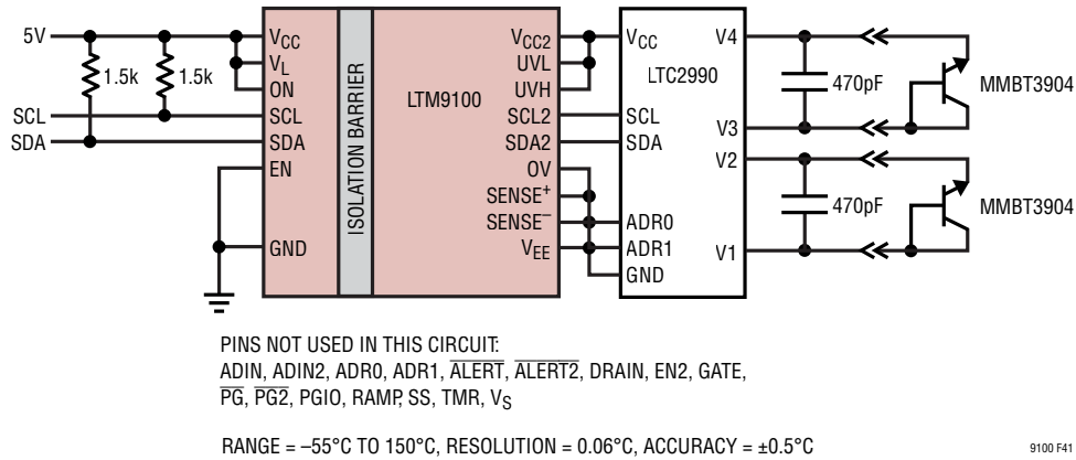
Figure 41. I²C Precision 14-Bit Remote (or Local) Dual Temperature Sense
