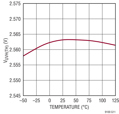
UVH Threshold vs Temperature
