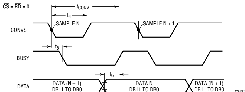
Figure 12. Mode 1a. \overline{CONVST} Starts a Conversion. Data Outputs Always Enabled. ( \overline{CONVST} = narrow pulse)
