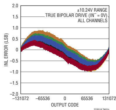
Integral Nonlinearity vs Output Code and Channel
