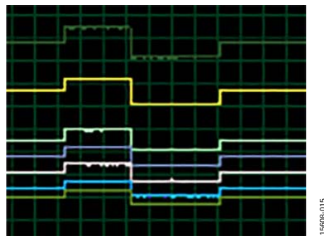
Figure 15. Rails Going from Nominal Setpoint to Margin High, Margin Low, and Back to Nominal Voltage
