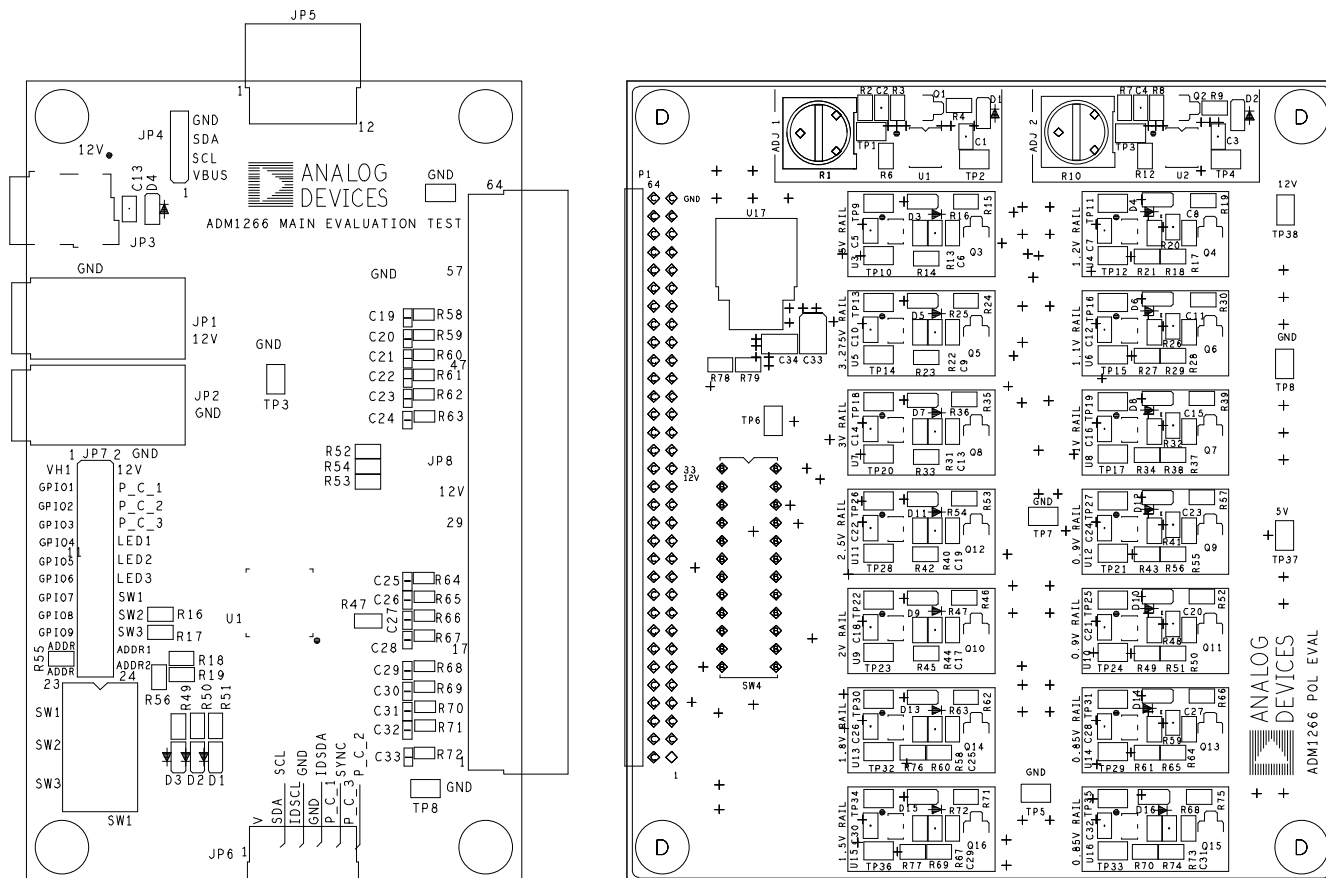
Figure 16. Top Silkscreen
