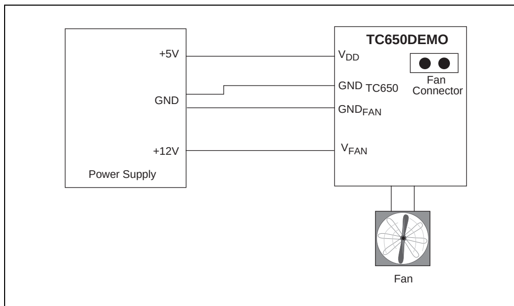
FIGURE 2-2: Typical Wiring Connections to Fan Module for 12V Fan and 5V Demo Board Supply
