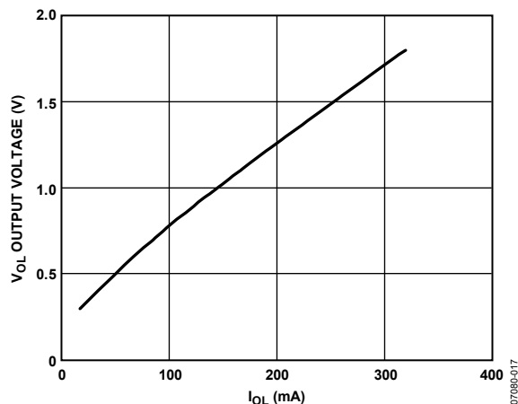
Figure 10. Typical V_{OL} vs. I_{OL} ( V_{DD1} = 5\text{ V} , V_{DD2} , V_{ISO} = 12\text{ V to }18\text{ V} )
