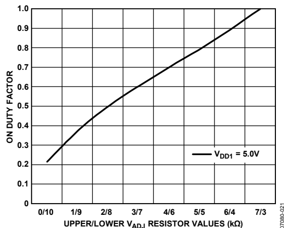
Figure 14. Upper/Lower V_{ADJ} Voltage Divider Resistor Values to Determine PWM Duty Factor for V_{DD1} = 5\text{ V}
