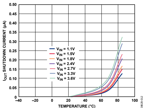
Figure 12. I_{OUT} Shutdown Current vs. Temperature, V_{OUT} = 0\text{ V}
