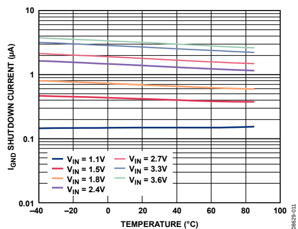
Figure 11. Shutdown Current vs. Temperature, V_{OUT} = 0\text{ V}
