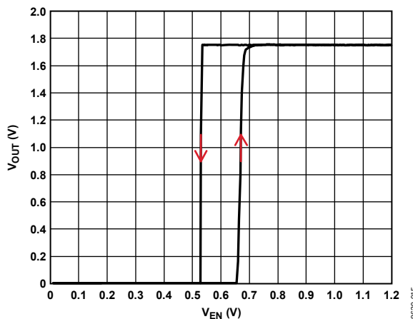
Figure 18. Typical EN Operation, V_{IN} = 1.8 V
