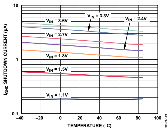
Figure 13. Reverse Shutdown Current vs. Temperature, V_{OUT} = 0\text{ V}
