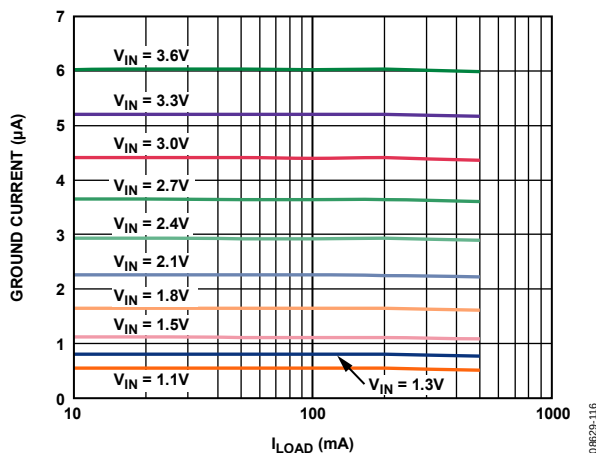
Figure 16. Ground Current vs. Load Current, Different Input Voltages
