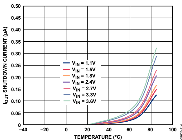
Figure 14. I_{OUT} Reverse Current vs. Temperature, V_{OUT} = 0\text{ V}
