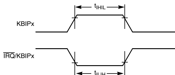
Figure 11. \overline{\text{IIRQ}} /KBIPx Timing
