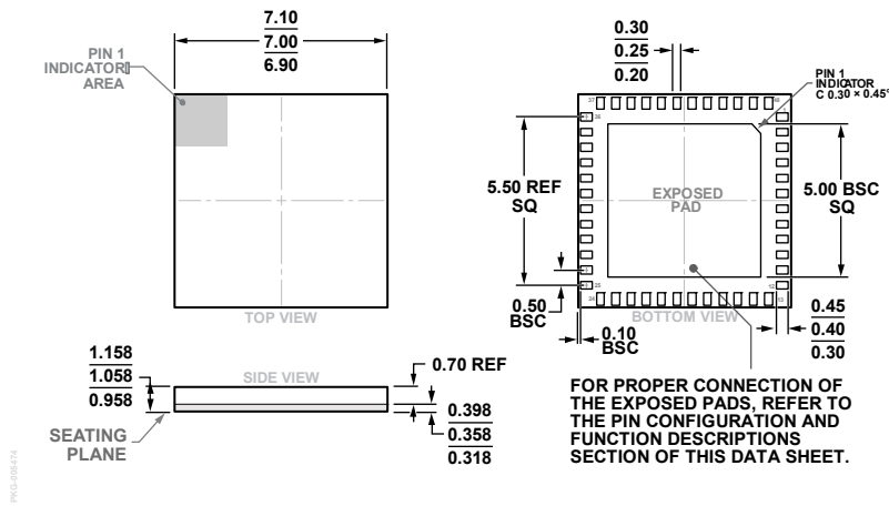
Figure 38. 48-Terminal Land Grid Array Package [LGA] (CC-48-4) Dimensions shown in millimeters
