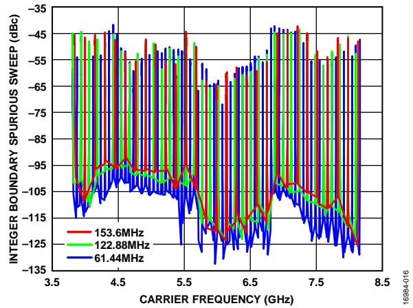
Figure 16. Integer Boundary Spurious Sweep vs. Carrier Frequency, f_{PFD} = 61.44 MHz, 122.88 MHz, and 153.6 MHz, Loop Filter Bandwidth = 100 kHz
