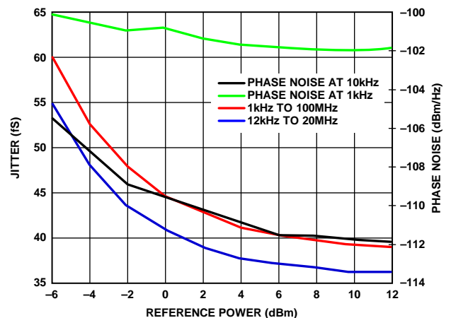
Figure 27. Jitter and Phase Noise, f_{PFD} = 250\ MHz
