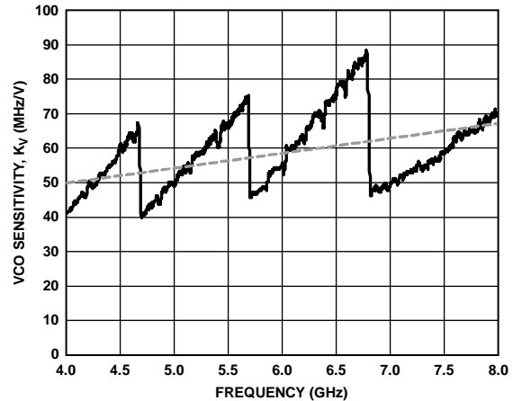
Figure 34. VCO Sensitivity, K_V vs. Frequency, VCC\_VCO = 3.3 V
