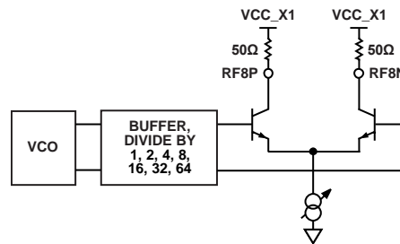
Figure 35. Output Stage
