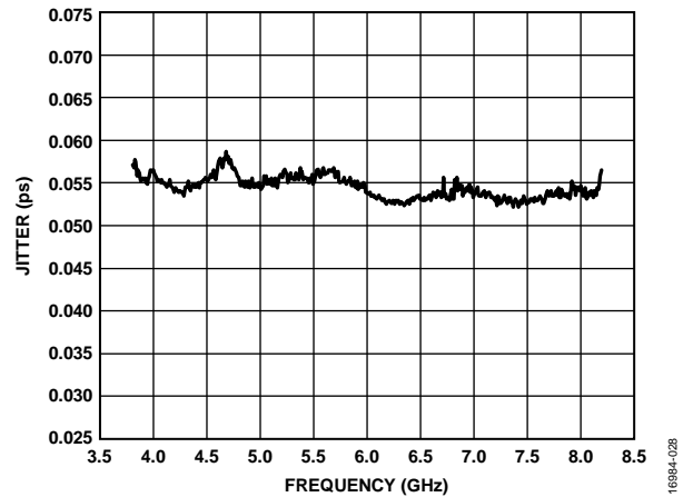
Figure 23. RMS Jitter Integrated from 1 kHz to 100 MHz, Fractional-N, f_{PFD} = 153.6 MHz, V_{CC\_VCO} = 3.3 V
