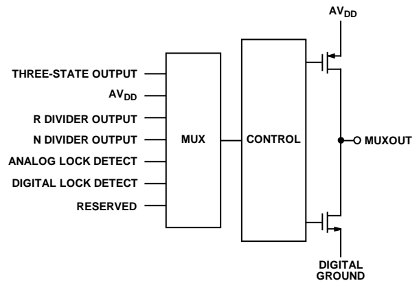
Figure 32. MUXOUT Schematic
