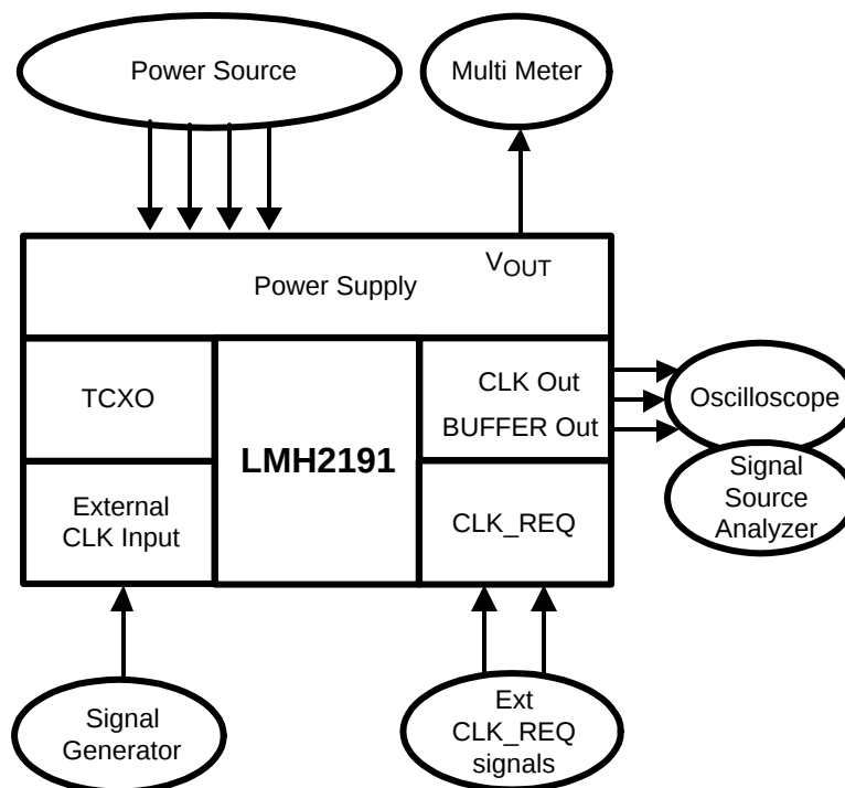
Figure 3. Test Setup
