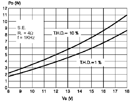
Figure 12. Output Power vs. Supply Voltage
