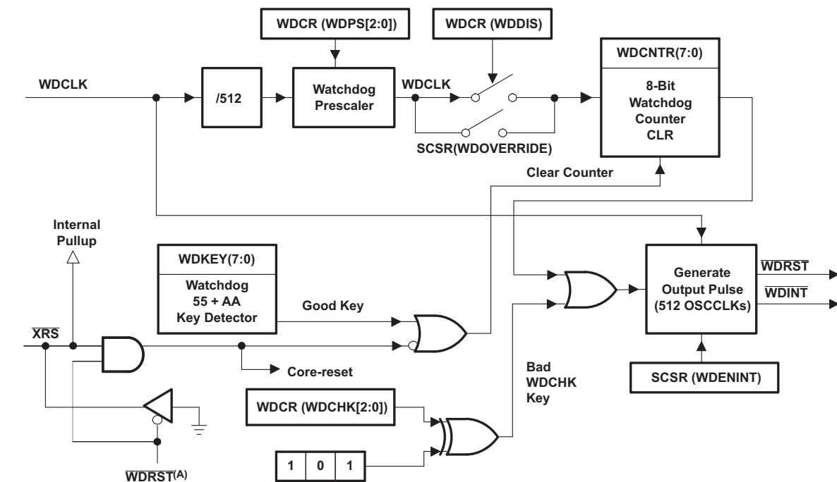
Figure 6-15. CPU Watchdog Module
