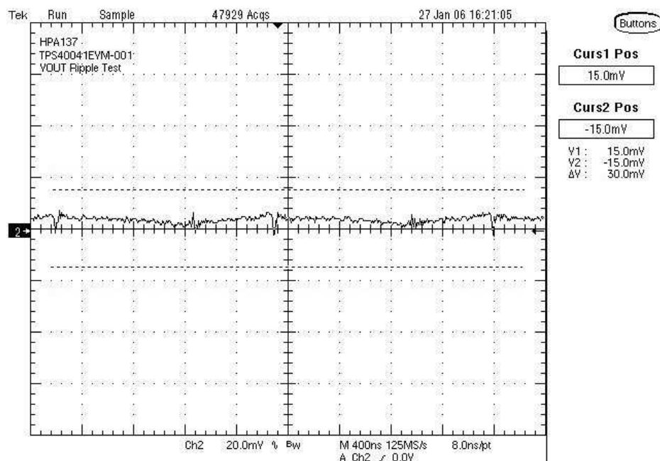
Figure 9. TPS40041EVM-001 Output Voltage Ripple, V_{IN} = 5.5 V, I_{OUT} = 6 A
