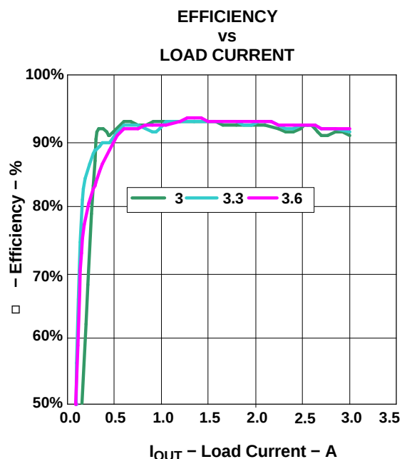
Figure 6. TPS40041EVM-001 Efficiency V_{IN} = 3.0 V to 3.6 V, V_{OUT} = 1.8 V, I_{OUT} = 0 A to 3 A
