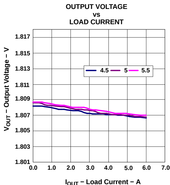
Figure 7. TPS40041EVM-001 Line and Load Regulation V_{IN} = 4.5 V to 5.5 V, V_{OUT} = 1.8 V, I_{OUT} = 0 A to 6 A
